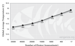
Global Average Temperature Vs. Number of Pirates
